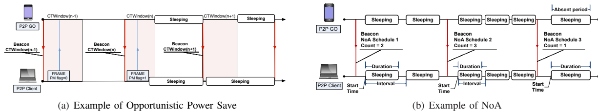
Fig. 3. P2P GO power saving protocols in Wi-Fi Direct.
